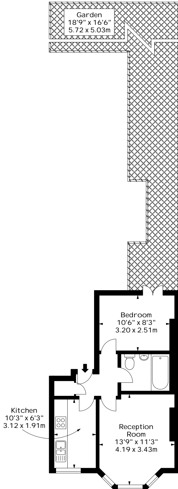
Ground Floor
